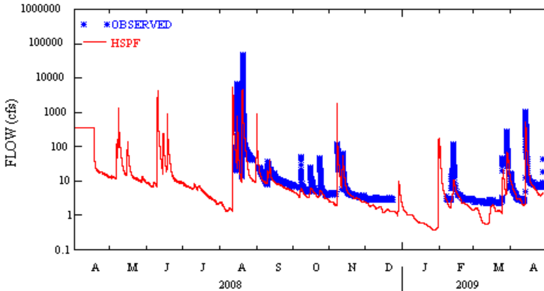
Figure A-24 Comparison of observed and simulated stream flows at L60 station
