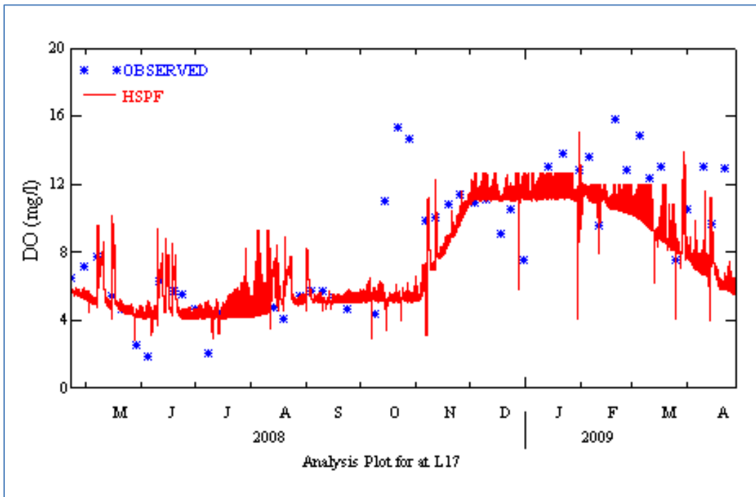
Figure 3-8 DO calibration plot at station L17
