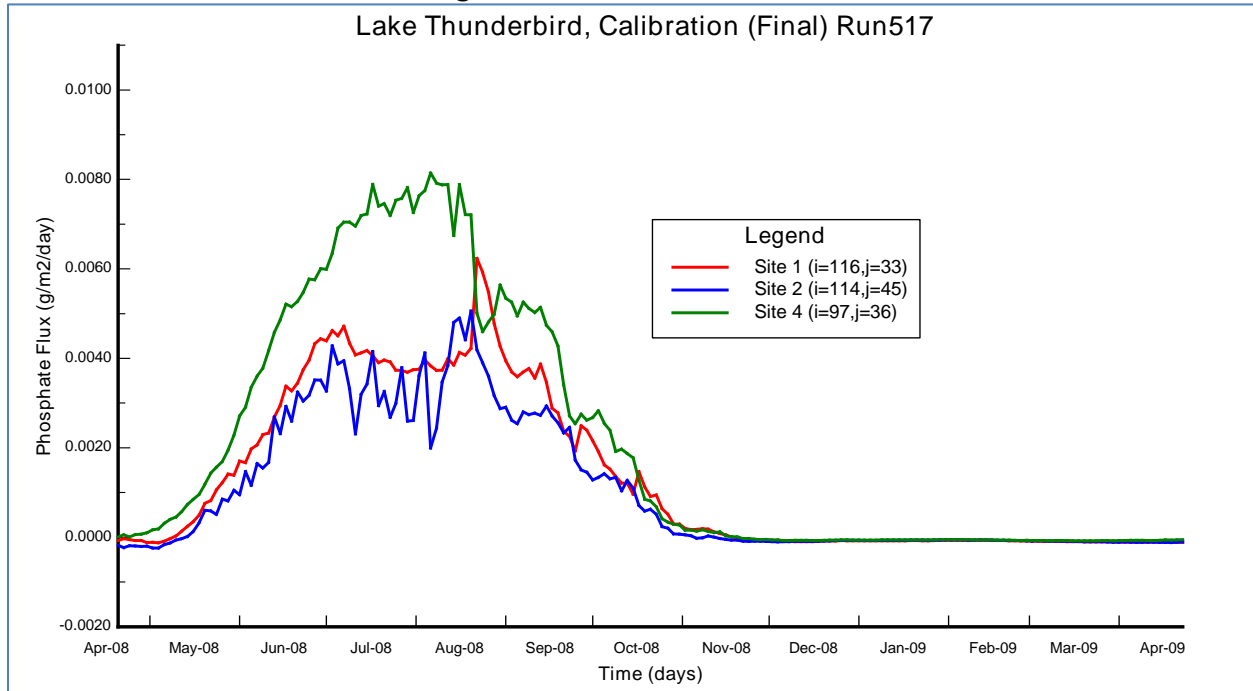
Figure B-14 Model Results for Benthic Flux of Dissolved Phosphate-P (PO 4 ) (as g/m 2 -day) for Sediment Diagenesis Model for Lacustrine Sites 1, 2 and 4.
